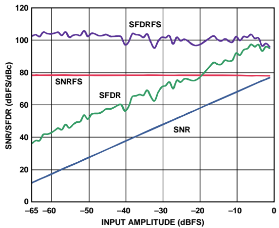
Figure 12. AD9266-80 SNR/SFDR vs. Input Amplitude (AIN) with f_{IN} = 9.7 MHz
