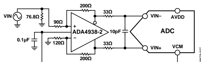
Figure 37. Differential Input Configuration Using the ADA4938-2
