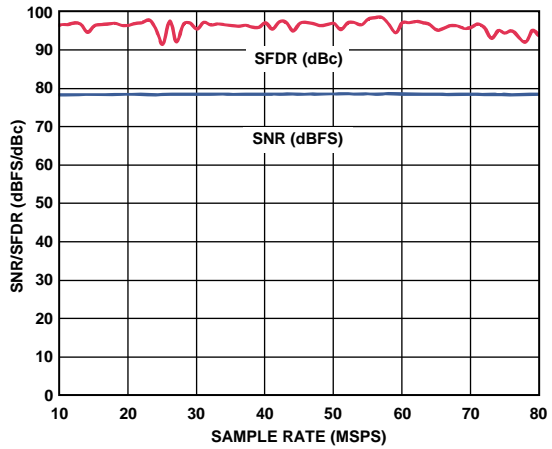
Figure 11. AD9266-80 SNR/SFDR vs. Sample Rate with AIN = 9.7 MHz
