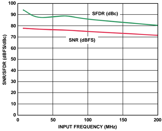
Figure 10. AD9266-80 SNR/SFDR vs. Input Frequency (AIN) with 2 V p-p Full Scale
