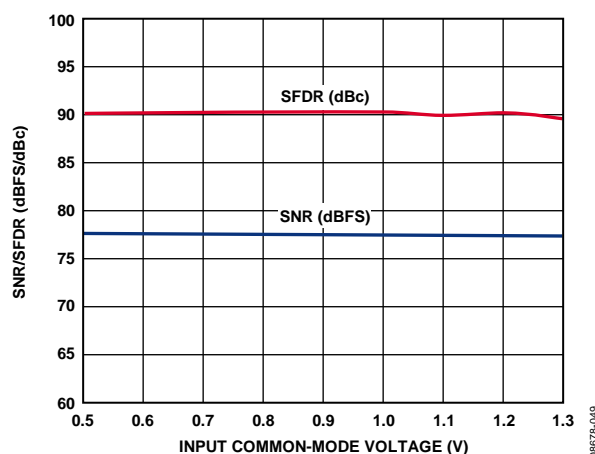
Figure 36. SNR/SFDR vs. Input Common-Mode Voltage, f_{IN} = 32.5 MHz, f_s = 80 MSPS
