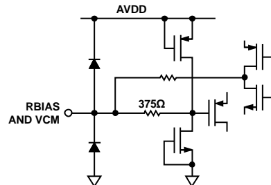
Figure 34. Equivalent RBIAS, VCM Circuit
