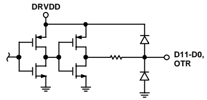
Figure 7. Equivalent Digital Output Circuit
