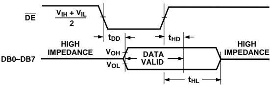
Figure 10. Read Timing
