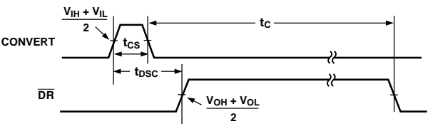
Figure 9. Convert Timing
