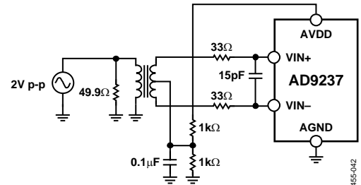
Figure 37. Differential Transformer-Coupled Configuration
