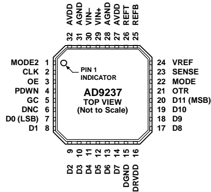
Figure 3. Pin Configuration
