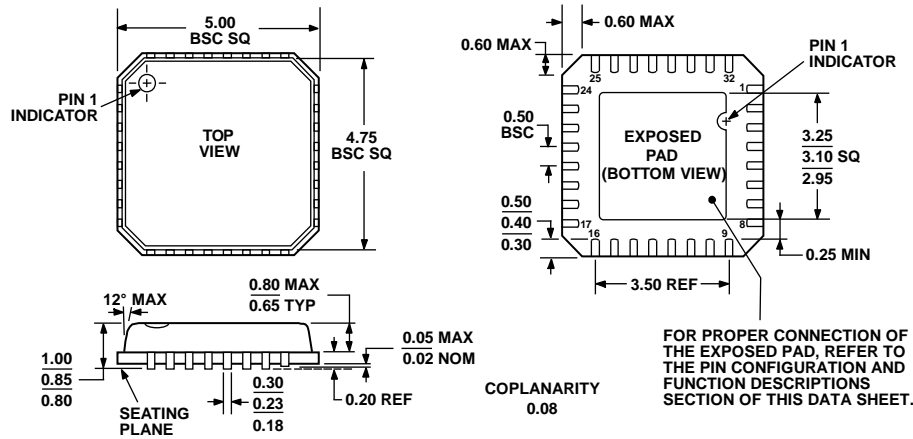
COMPLIANT TO JEDEC STANDARDS MO-220-VHHD-2 Figure 47. 32-Lead Lead Frame Chip Scale Package [LFCSP_VQ] 5 mm × 5 mm Body, Very Thin Quad (CP-32-2) Dimensions shown in millimeters
