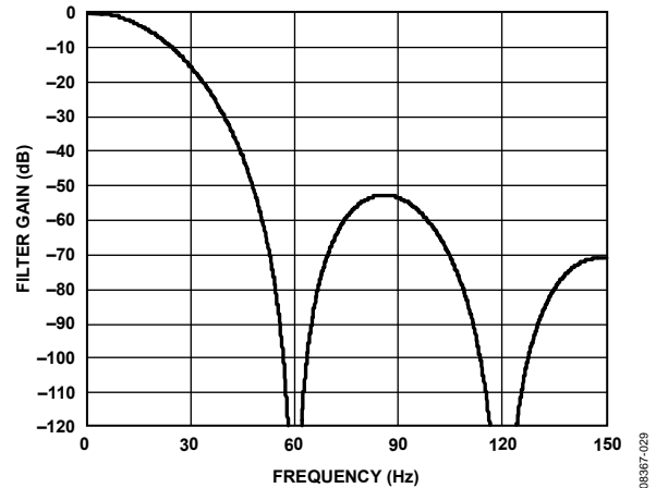
Figure 33. Sinc 4 Filter Response (FS[9:0] = 80)
