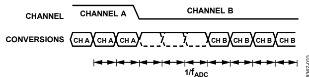
Figure 37. Sinc 3 Channel Change
