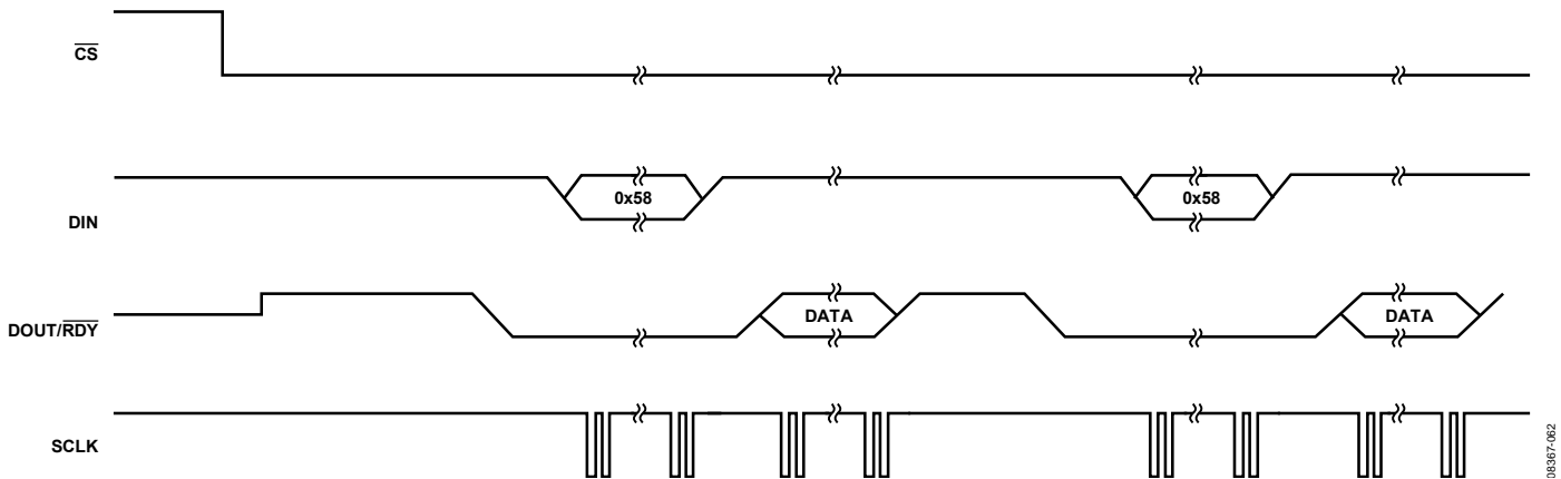
Figure 26. Continuous Conversion
