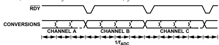
Figure 24. Channel Sequencer
