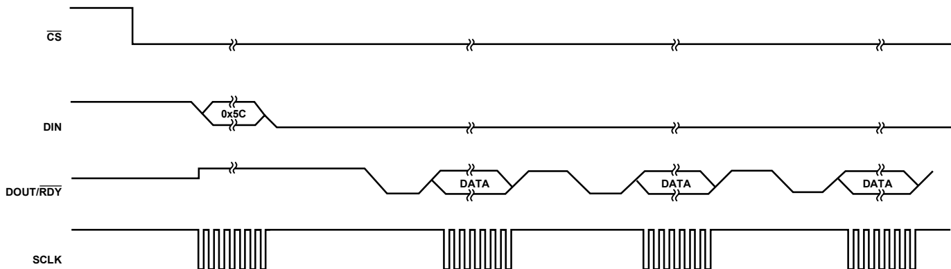
Figure 27. Continuous Read
