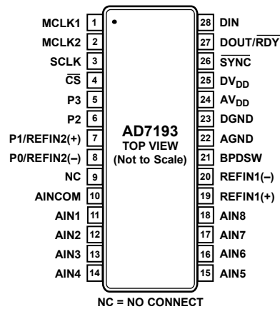
Figure 5. 28-lead TSSOP Pin Configuration
