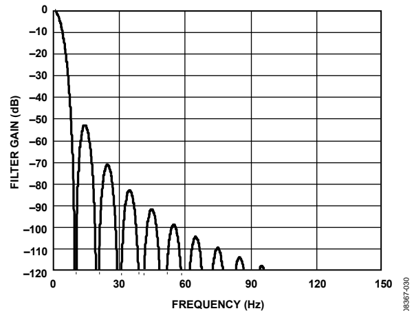
Figure 34. Sinc 4 Filter Response (FS[9:0] = 480)
