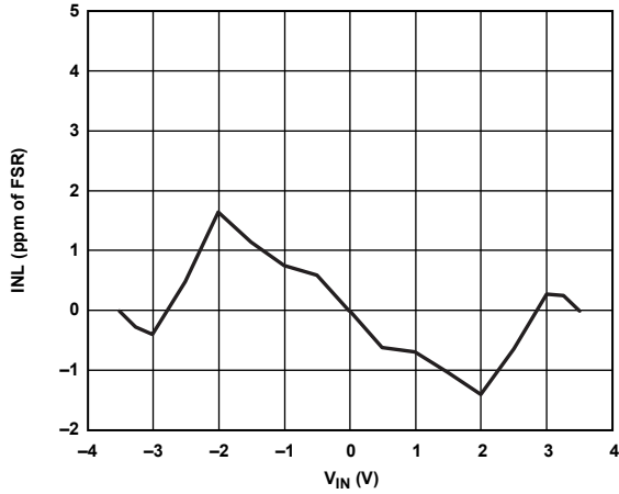
Figure 13. INL (Gain = 1)
