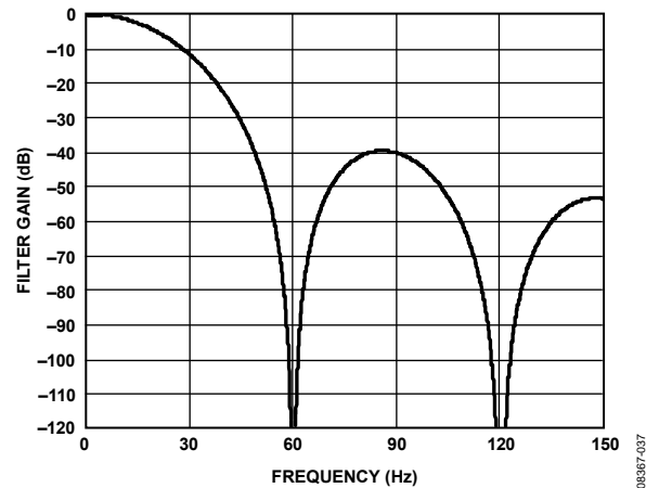
Figure 41. Sinc 3 Filter Response (FS[9:0] = 80)
