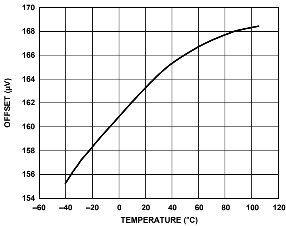
Figure 15. Offset vs. Temperature (Gain = 1, Chop Disabled)
