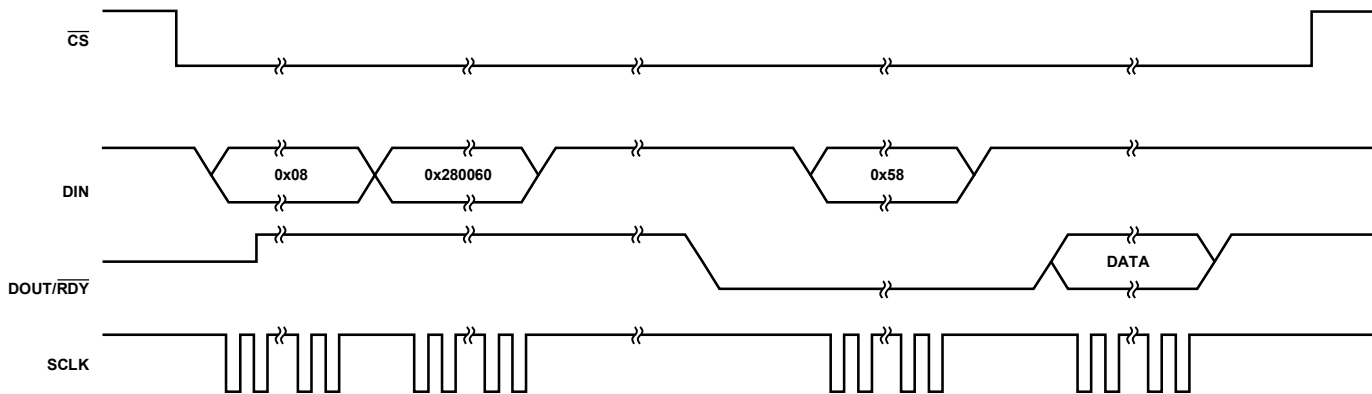
Figure 25. Single Conversion
