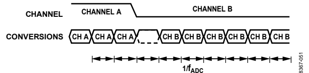
Figure 55. Fast Settling, Sinc 4 Filter
