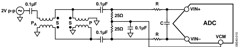
Figure 40. Differential Double Balun Input Configuration
