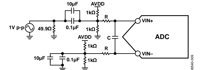
Figure 39. Single-Ended Input Configuration
