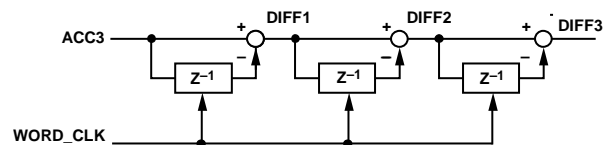
Figure 27. Differentiator
