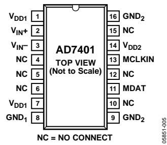
Figure 5. Pin Configuration
