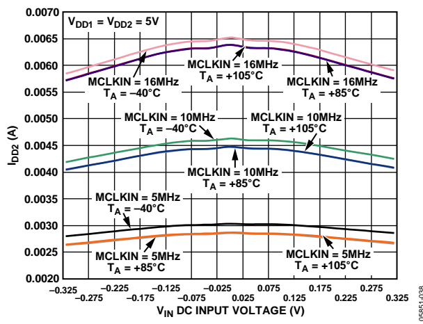
Figure 17. I DD2 vs. V IN at Various Temperatures
