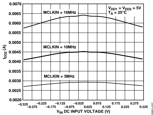
Figure 16. I DD2 vs. V IN DC Input Voltage
