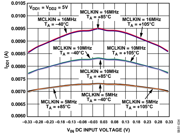
Figure 15. I DD1 vs. V IN at Various Temperatures
