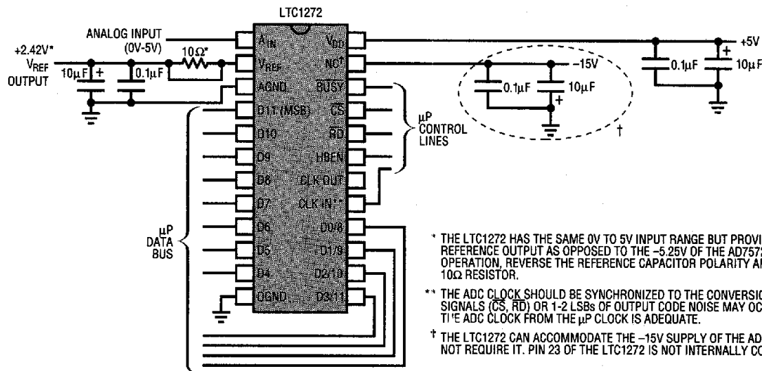
Figure 22. Plugging the LTC1272 into an AD7572 Socket Case 1: Clock Synchronous with \overline{CS} and \overline{RD}
