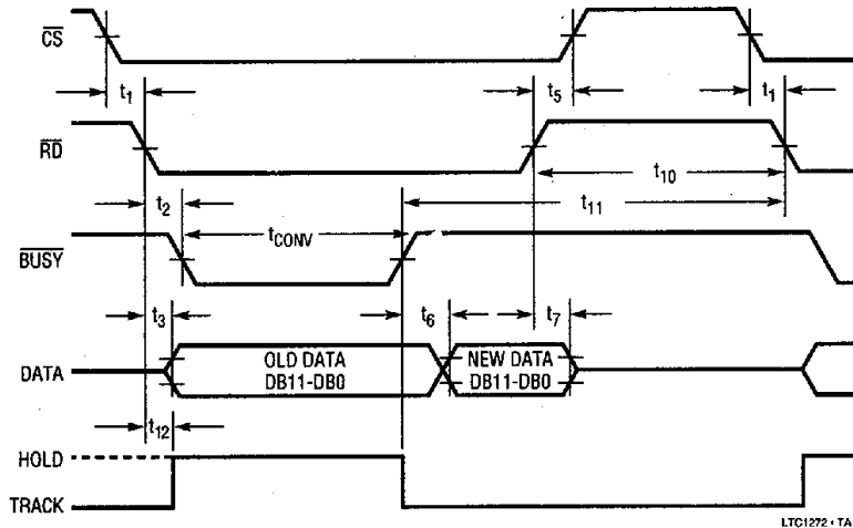
Figure 14. Slow Memory Mode, Parallel Read Timing Diagram
