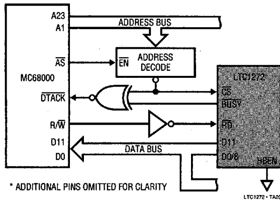
Figure 18. LTC1272 MC68000 Interface
