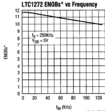
LT1272-TPC07
