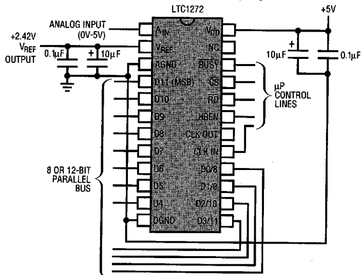
Single 5V Supply, 3μs, 12-Bit Sampling ADC
