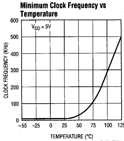
LT1272-TPC04
