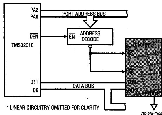
Figure 20. LTC1272 TMS32010 Interface
