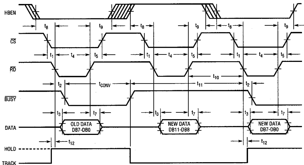
Figure 17. ROM Mode, Two Byte Read Timing Diagram
