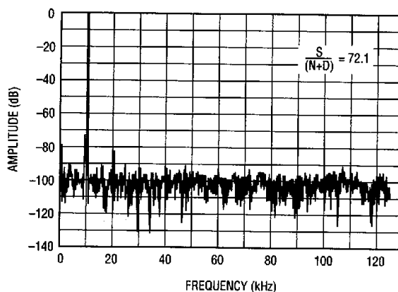
1024 Point FFT, f_s = 250\text{kHz} , f_{IN} = 10\text{kHz}
