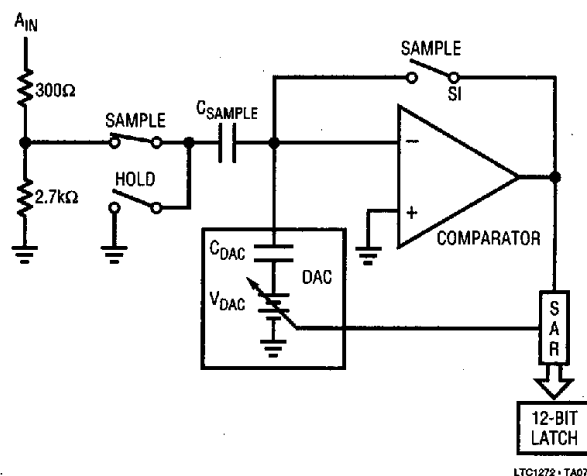
Figure 1. A_{IN} Input
