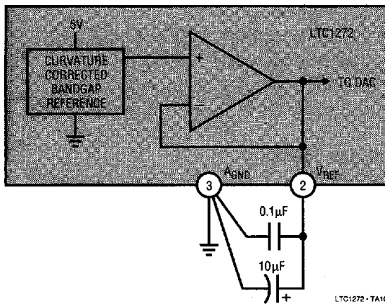
Figure 8. LTC1272 Internal 2.42V Reference
