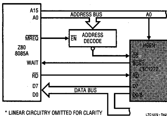
Figure 19. LTC1272 8085A/Z80 Interface
