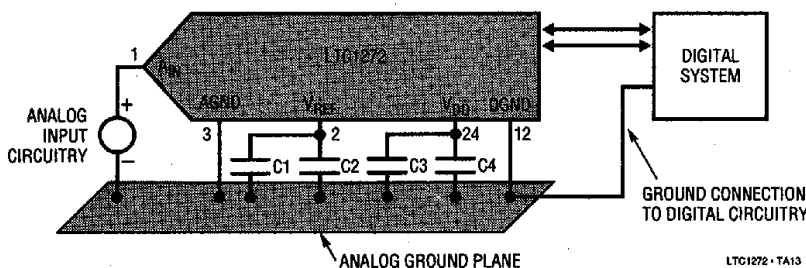
Figure 11. Power Supply Grounding Practice
