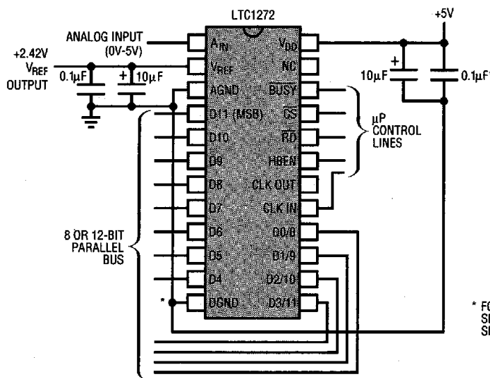
Figure 21. Single 5V Supply, 3μs, 12-Bit Sampling ADC
