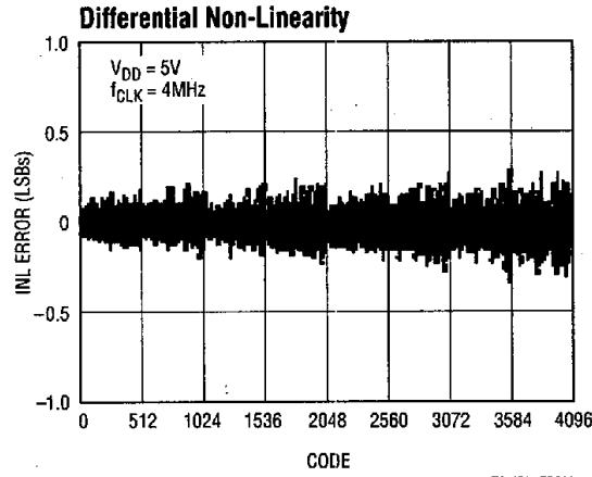
LTC1272-TPC02
