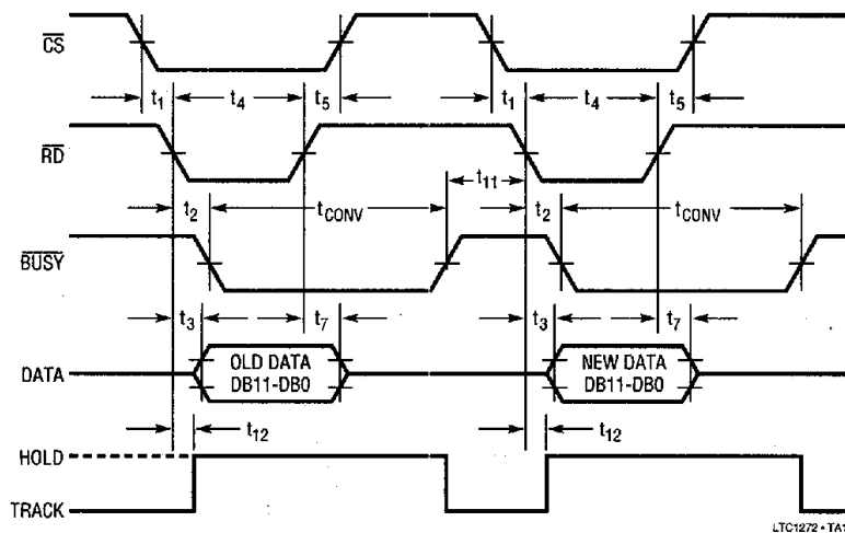
Figure 16. ROM Mode, Parallel Read Timing Diagram
