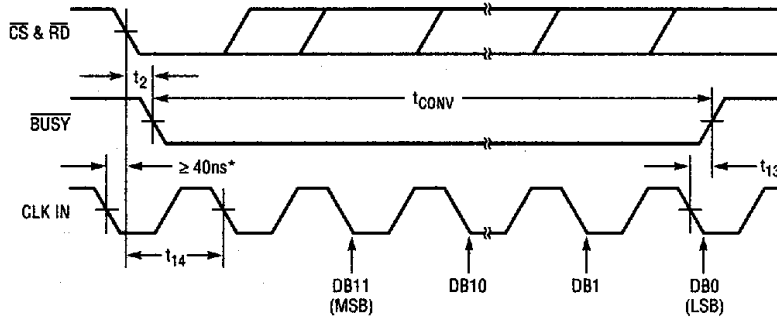
Figure 5. RD and CLK IN for Synchronous Operation
