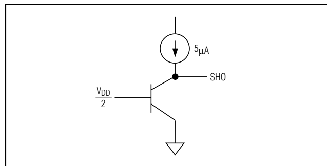
Figure 7. SHO Output Circuit
