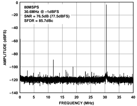
Figure 9. AD9269-80 Single-Tone FFT with f_{IN} = 30.6 MHz
