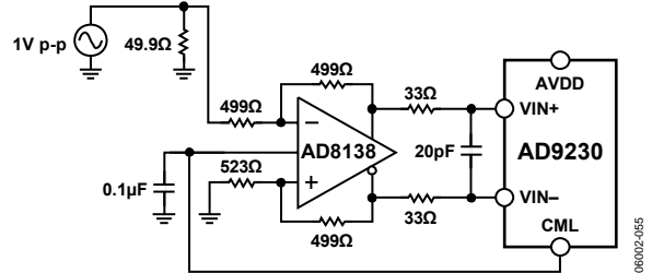
Figure 52. Differential Input Configuration Using the AD8138
