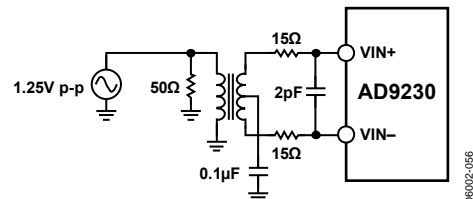
Figure 53. Differential Transformer—Coupled Configuration
