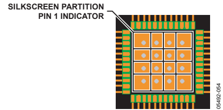
Figure 58. Typical PCB Layout
