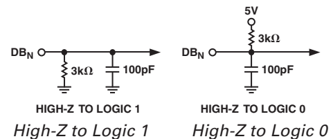
Figure 3a. Load Circuit for Access Time Test
