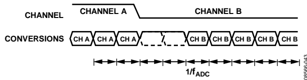
Figure 44. Channel Change ( Sinc^4 Chop Enabled)
