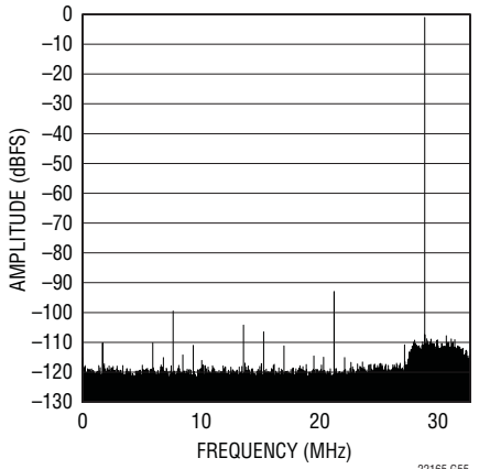
LTC2215 64k Point FFT, f_{IN} = 28.7\text{MHz} , -1dBFS
