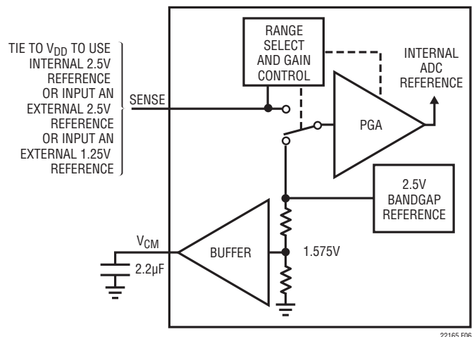
Figure 6. Reference Circuit
