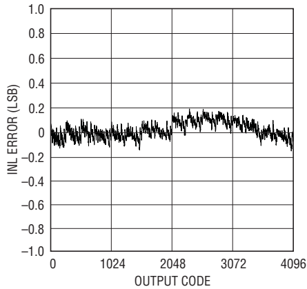
LTC2175-12: Integral Nonlinearity (INL)
