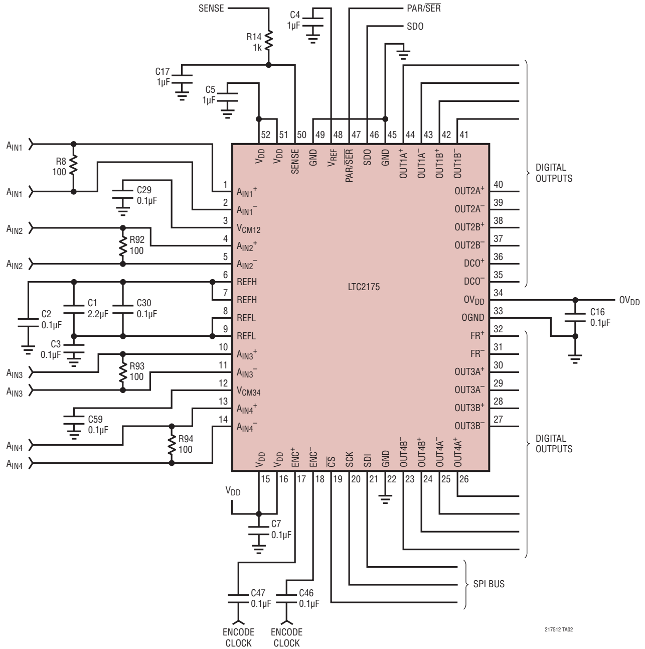
LTC2175 Schematic
