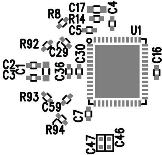
Silkscreen Top
