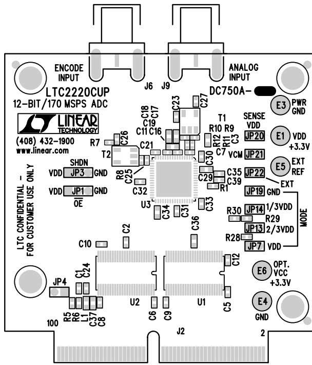
Silkscreen Top
