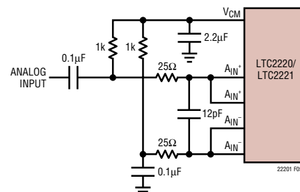
Figure 5. Single-Ended Drive
