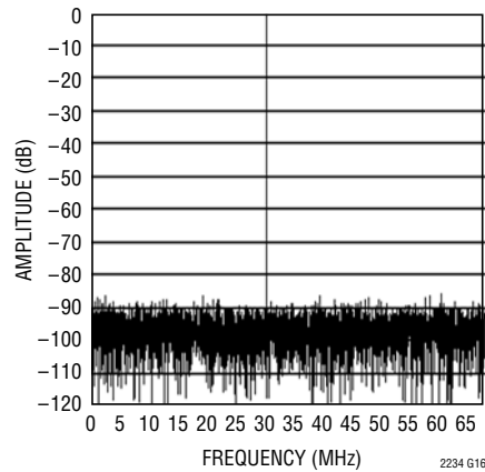
LTC2234: 8192 Point FFT, f_{IN} = 30\text{MHz} , -1dB, 1V Range
