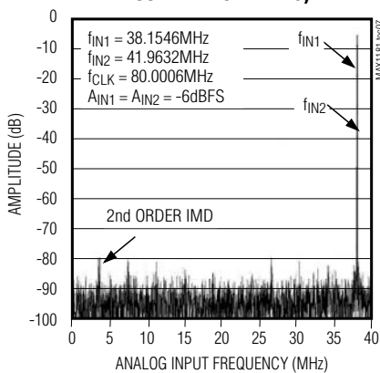
TWO-TONE IMD PLOT (8192-POINT RECORD, COHERENT SAMPLING)
