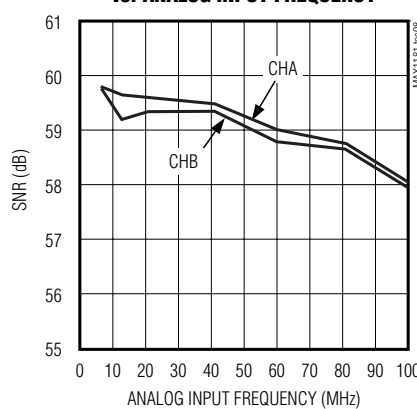
SIGNAL-TO-NOISE RATIO vs. ANALOG INPUT FREQUENCY
