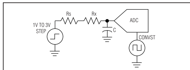
Figure 2. Test Circuit
