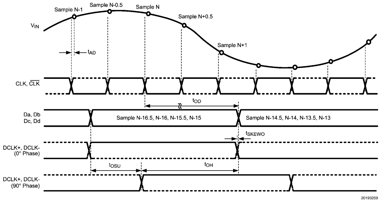
FIGURE 4. ADC083000 Timing — DDR Clcking
