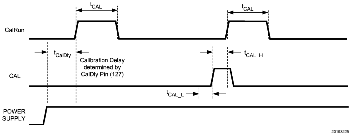
FIGURE 8. Calibration and On-Command Calibration Timing
