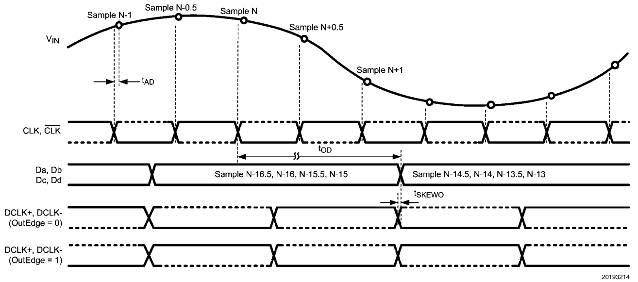
FIGURE 3. ADC083000 Timing — SDR Clcking
