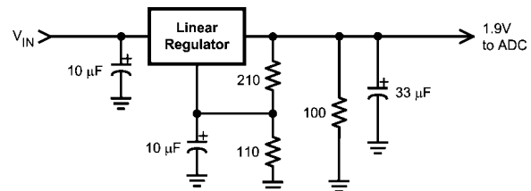
FIGURE 16. Non-Spiking Power Supply
