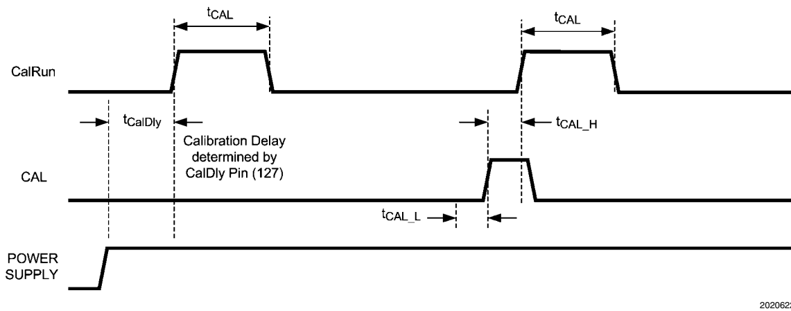
FIGURE 10. Power-up Calibration and On-Command Calibration Timing
