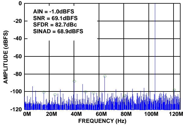
FIGURE 17. SINGLE-TONE SPECTRUM @ 105MHz
