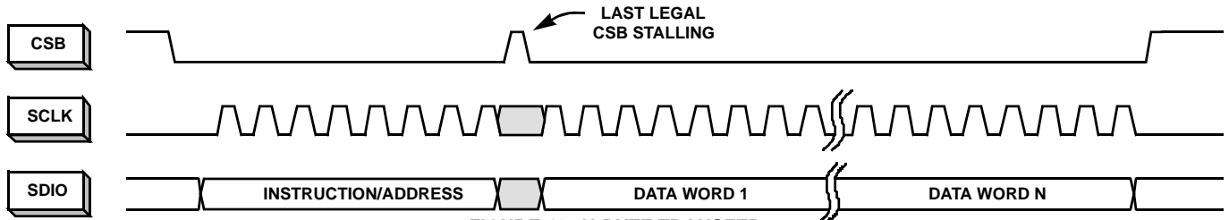
FIGURE 40. N-BYTE TRANSFER
