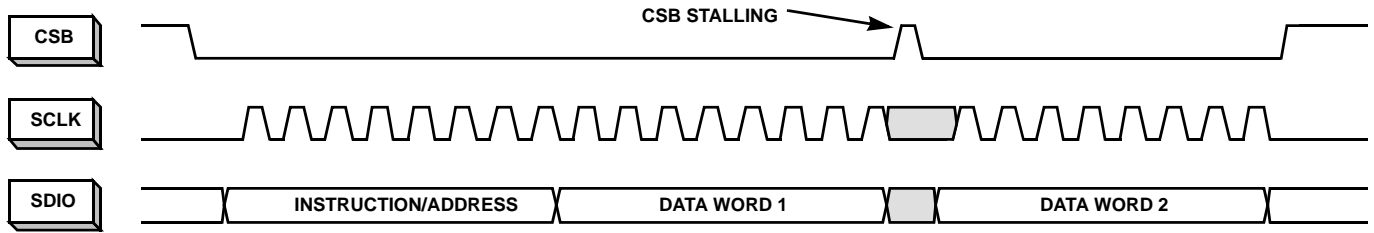
FIGURE 39. 2-BYTE TRANSFER
