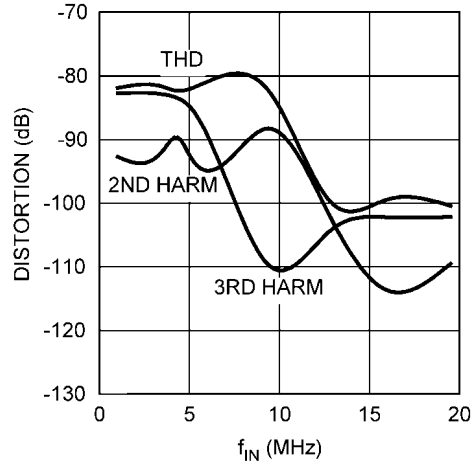
Distortion vs f_{IN} , f_{CLK} = 40MHz , IOR off
