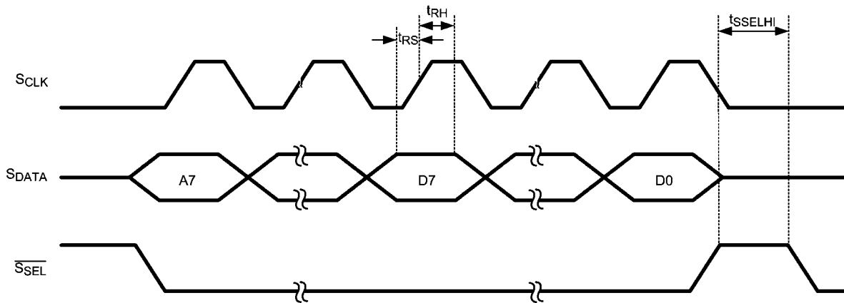
FIGURE 4. SPI Read Timing
