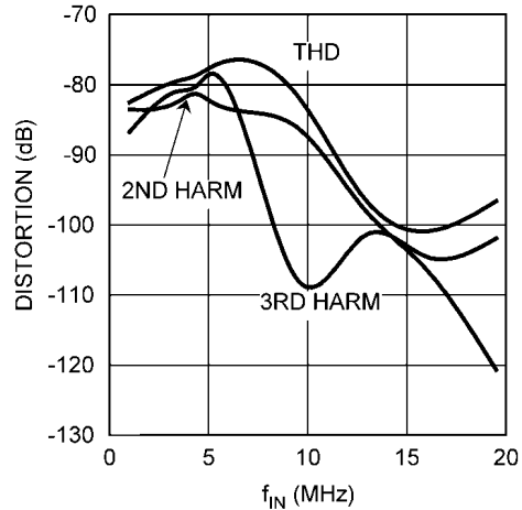
Distortion vs f_{IN} , f_{CLK} = 40MHz , IOR on
