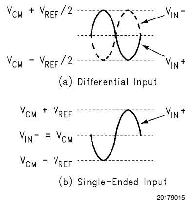
FIGURE 2. Expected Input Signal Range
