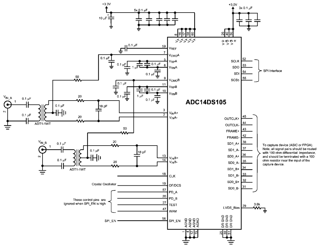
FIGURE 9. Application Circuit
