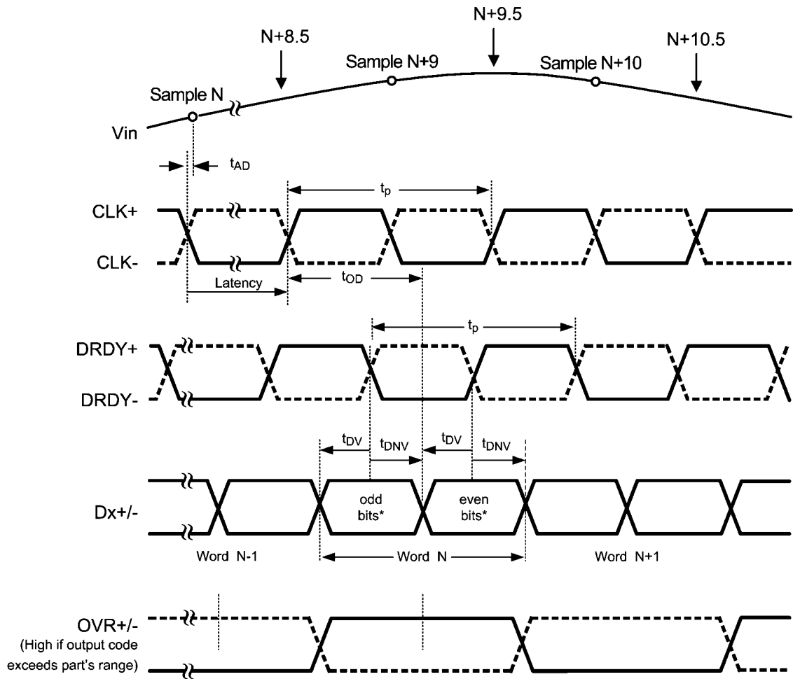
Output Timing
