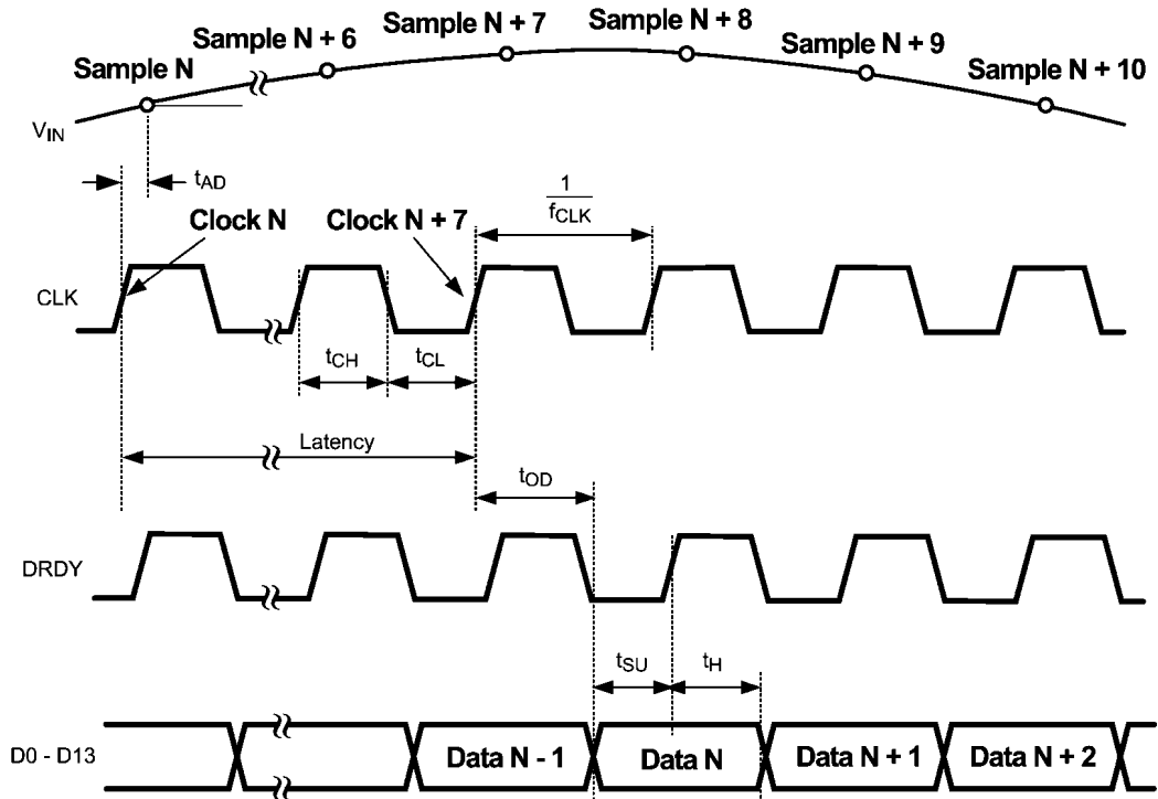
FIGURE 1. Output Timing
