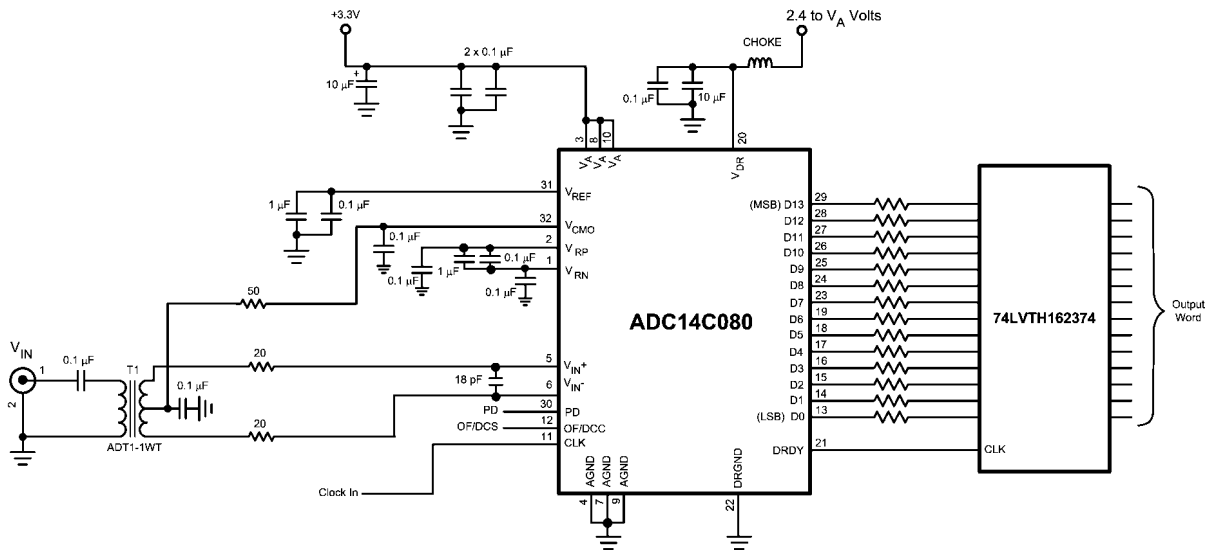
FIGURE 7. Application Circuit
