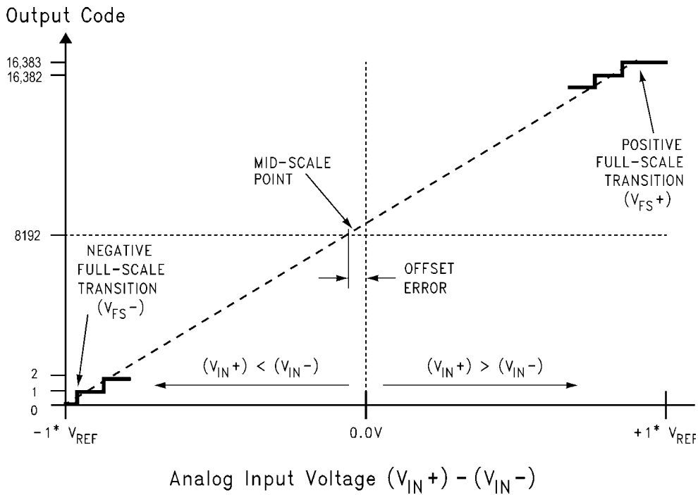
FIGURE 2. Transfer Characteristic
