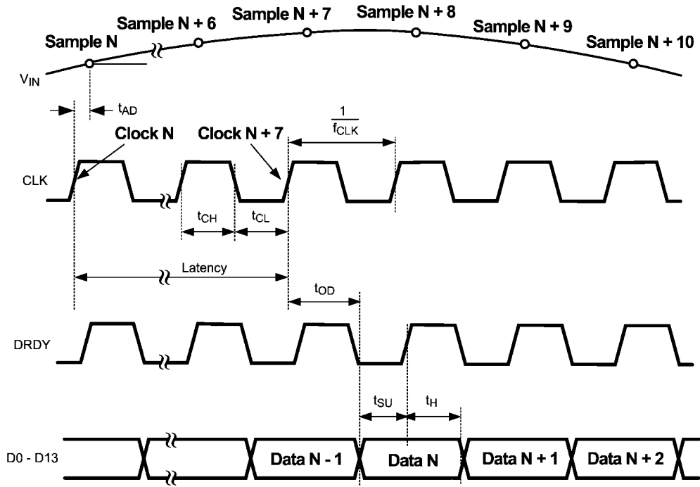
FIGURE 1. Output Timing
