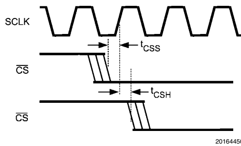
FIGURE 3. SCLK and \overline{CS} Timing Parameters
