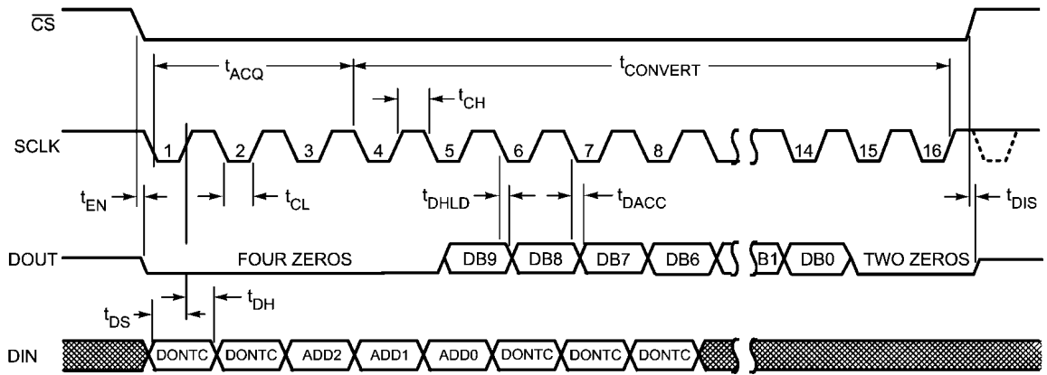
FIGURE 2. ADC108S022 Serial Timing Diagram
