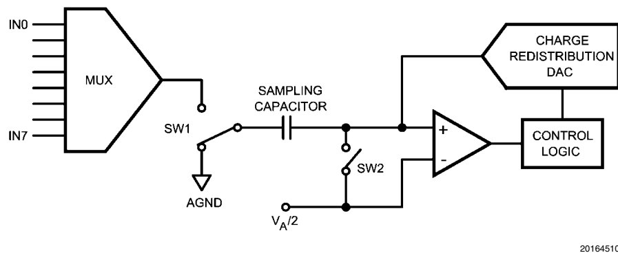
FIGURE 5. ADC108S022 in Hold Mode
