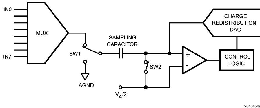
FIGURE 4. ADC108S022 in Track Mode
