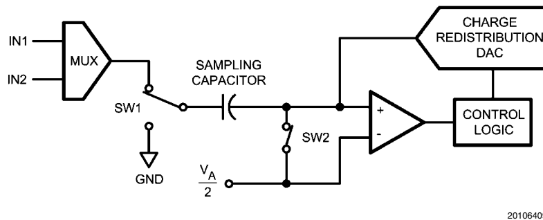
FIGURE 1. ADC122S051 in Track Mode
