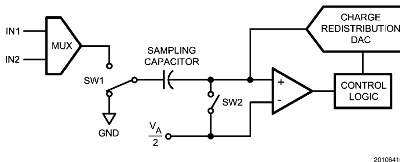
FIGURE 2. ADC122S051 in Hold Mode
