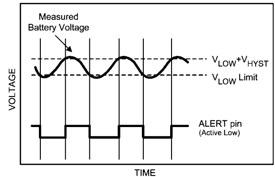
FIGURE 23. Trickle Charge
