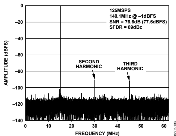
Figure 33. AD9265-125 Single-Tone FFT with f_{IN} = 140.1 MHz
