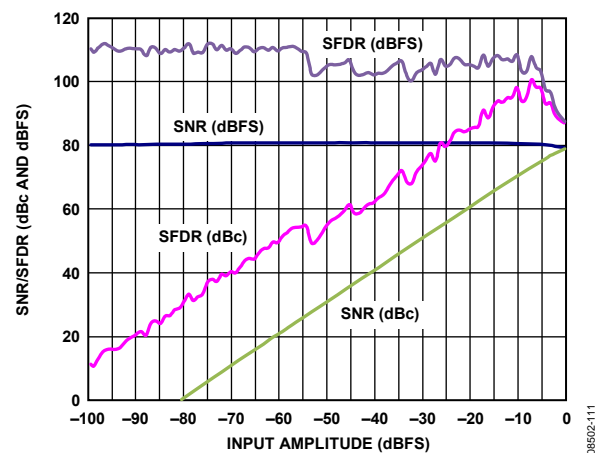
Figure 11. AD9265-80 Single-Tone SNR/SFDR vs. Input Amplitude ( A_{IN} ) with f_{IN} = 98.12 MHz
