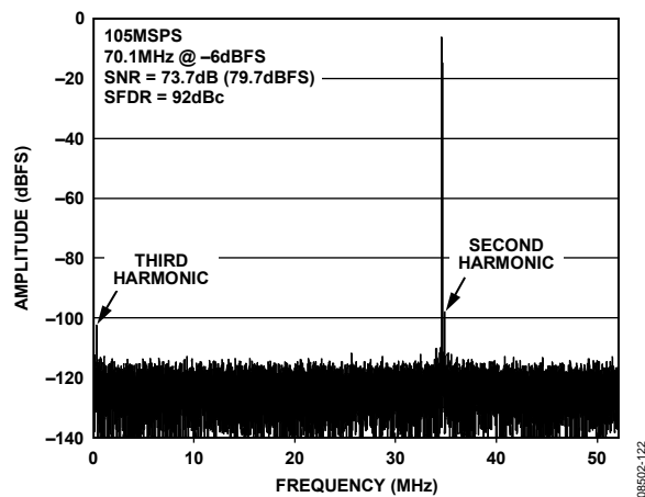
Figure 22. AD9265-105 Single-Tone FFT with f_{IN} = 70.1 MHz @ -6dBFS with Dither Enabled
