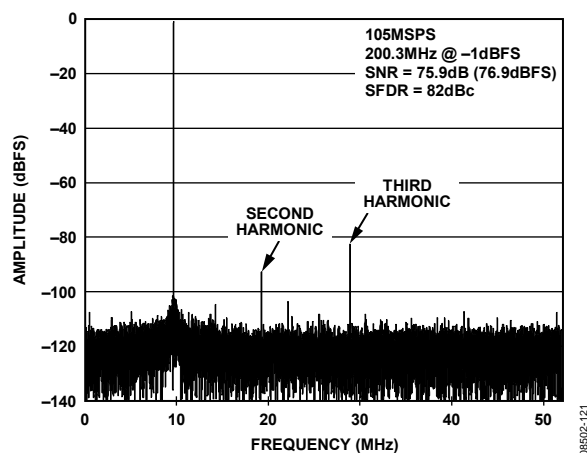
Figure 21. AD9265-105 Single-Tone FFT with f_{IN} = 200.3 MHz
