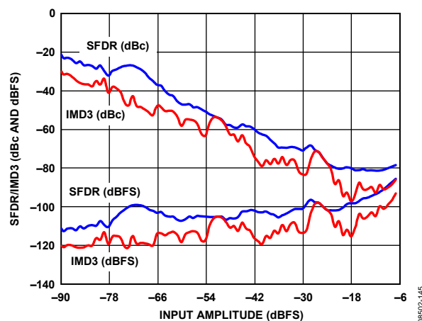
Figure 45. AD9265-125 Two-Tone SFDR/IMD3 vs. Input Amplitude ( A_{IN} ) with f_{IN1} = 169.1 MHz, f_{IN2} = 172.1 MHz, f_s = 125 MSPS
