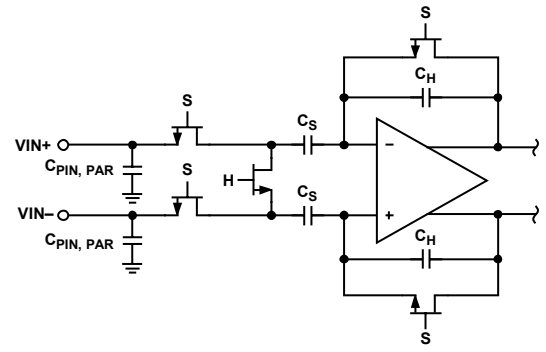
Figure 36. Switched Capacitor SHA Input
