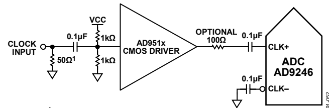
Figure 50. Single-Ended 3.3 V CMOS Sample Clock
