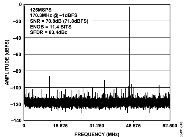
Figure 17. AD9246-125 Single-Tone FFT with f_{IN} = 170.3 MHz
