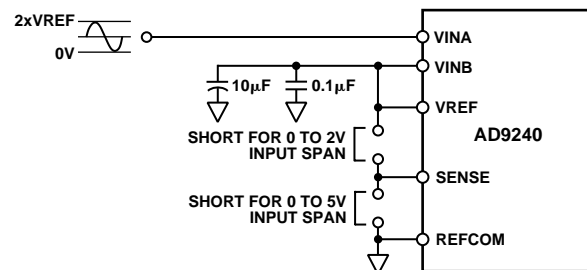
Figure 39. Internal Reference (2 V p-p Input Span, V CM = 1 V, or 5 V p-p Input Span, V CM = 2.5 V)
