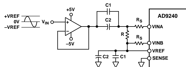
Figure 37. AC-Coupled Input
