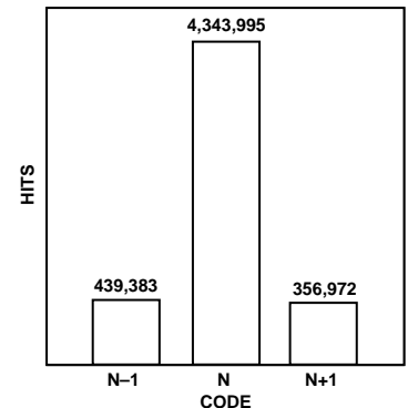
Figure 13. "Grounded-Input" Histogram (Input Span = 5 V)
