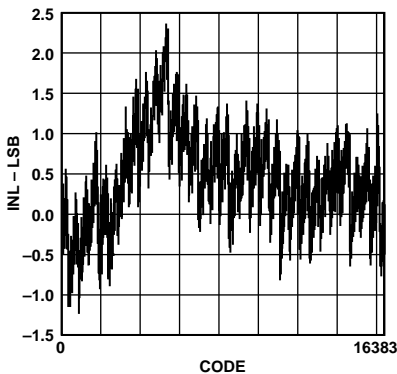
Figure 11. Typical INL (Input Span = 5 V)
