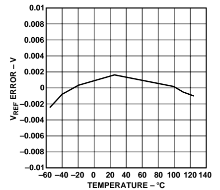
Figure 19. Typical Voltage Reference Error vs. Temperature
