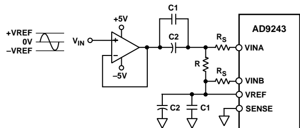
Figure 34. AC-Coupled Input
