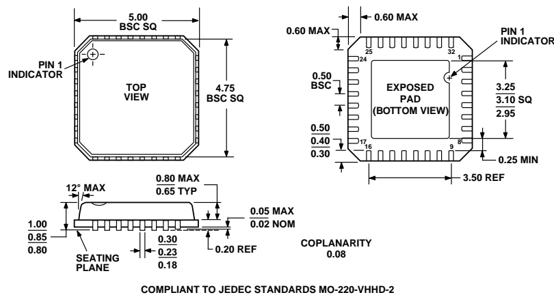
Figure 64. 32-Lead Lead Frame Chip Scale Package [LFCSP] 5 mm x 5 mm Body (CP-32-2) Dimensions shown in millimeters
