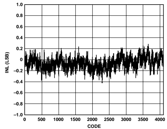
Figure 31. Typical INL
