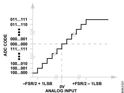
Figure 19. Transfer Characteristic
