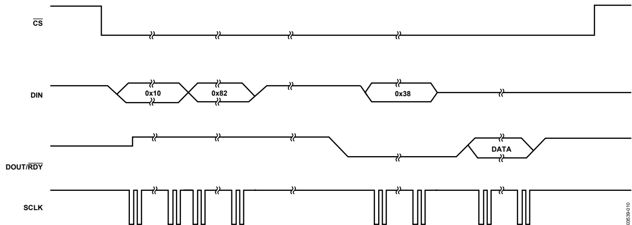
Figure 11. Single Conversion
