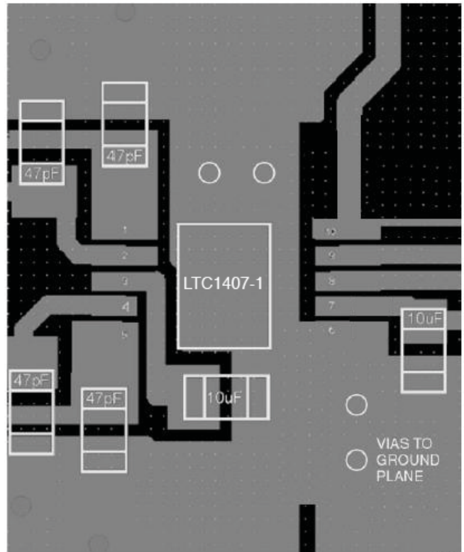
Figure 7. Recommended Layout
