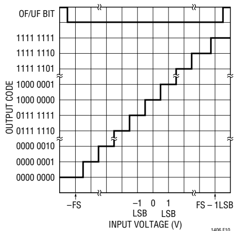
Figure 10. Transfer Characteristics
