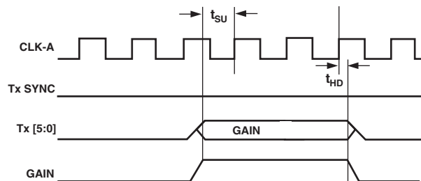
Figure 6. GAIN Programming
