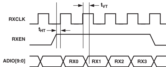
Figure 4. Receive Data Output Timing Diagram
