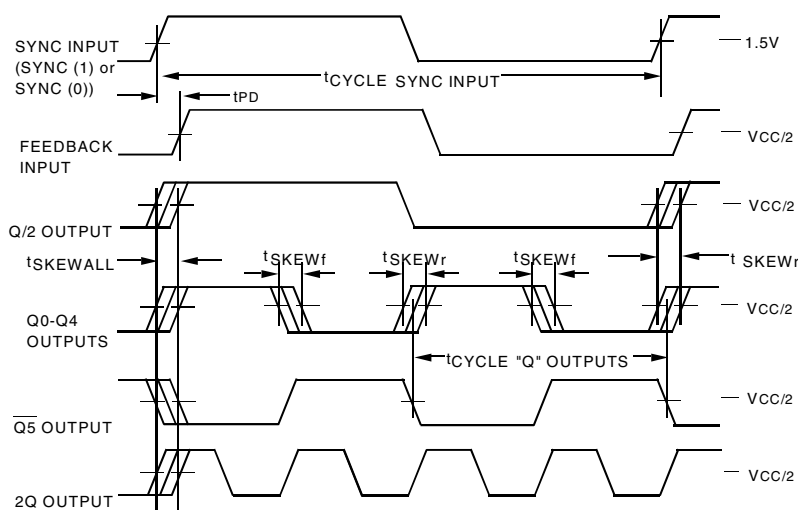
Propagation Delay, Output Skew
