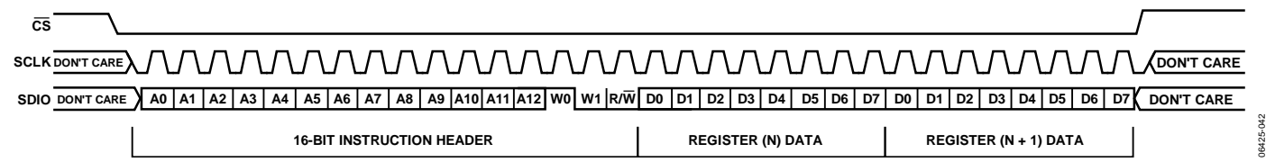
Figure 67. Serial Control Port Write—LSB First, 16-Bit Instruction, Two Bytes Data
