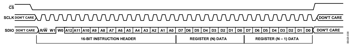
Figure 63. Serial Control Port Write—MSB First, 16-Bit Instruction, Two Bytes Data
