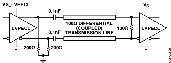
Figure 72. AC-Coupled LVPECL with Parallel Transmission Line
