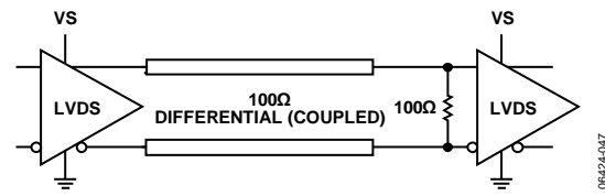
Figure 73. LVDS Output Termination
