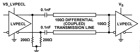
Figure 54. AC-Coupled LVPECL with Parallel Transmission Line
