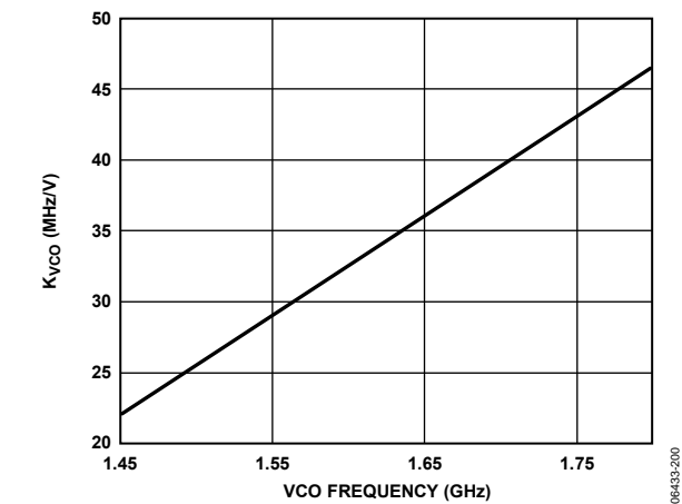
Figure 6. K_{VCO} vs. VCO Frequency
