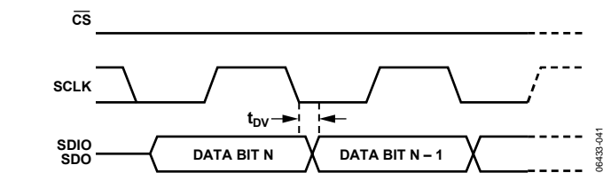
Figure 48. Serial Control Port Timing Diagram—Read
