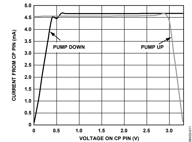
Figure 7. Charge Pump Characteristics @ V_{CP} = 3.3 V
