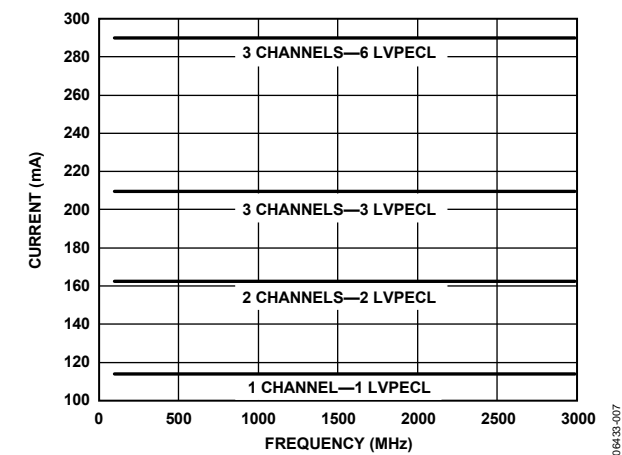
Figure 5. Current vs. Frequency, Direct-to-Output, LVPECL Outputs
