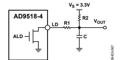
Figure 34. Example of Analog Lock Detect Filter Using an N-Channel Open-Drain Driver
